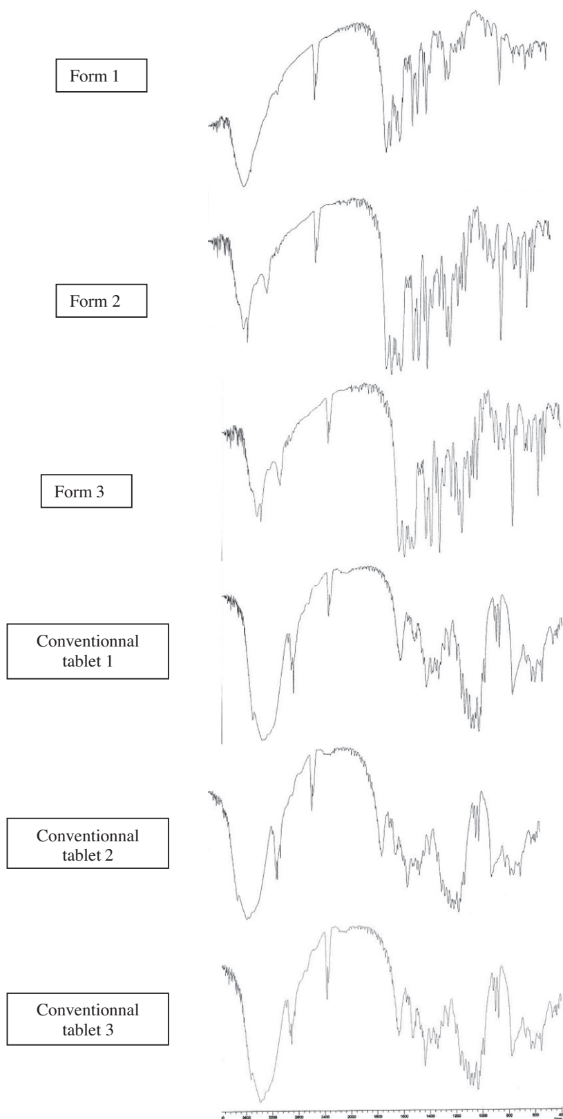
Figure 13 IR spectra of Piroxicam polymorphs and their conventional forms.
