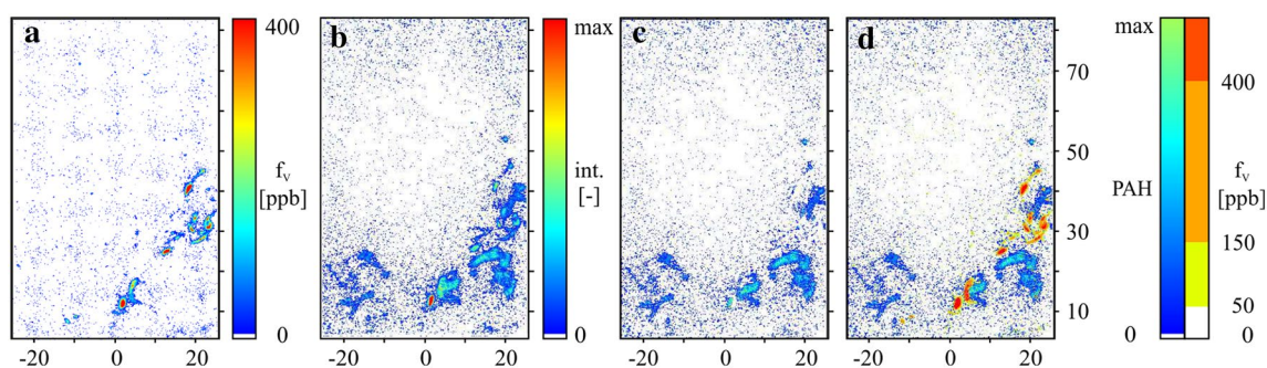
Fig. 3 Analysis of PAH LIF images ( b ) excited in the UV by subtraction of the simultaneously IR-excited soot ( a ) to yield an image consisting of pure PAH ( c ), and addition of the color-coded soot distribution ( d ). The image size corresponds to the area excited by the
