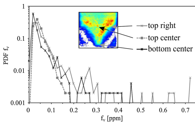
Fig. 9 Probability density functions of soot concentrations found along the soot formation region compared to the central inner recirculation zone in the absence of oxidation. For the top center position, no soot concentrations above 0.2 ppm are identified
