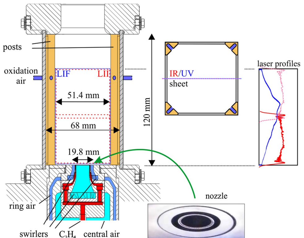
Fig. 1 Burner geometry, nozzle details and cross section at the height of oxidation air injection, with the laser sheet positions and profiles inserted at top right; blue indicates the UV sheet profile, red represents the IR sheet profile in both positions
