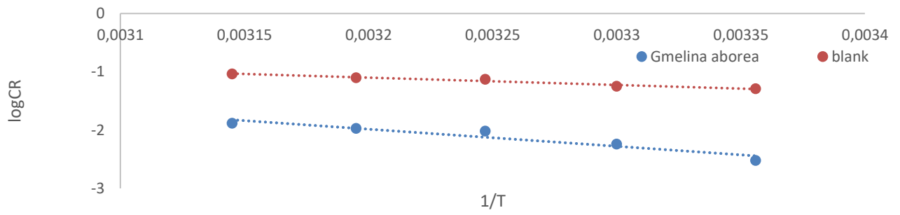
Figure 1. Arrhenius plot
