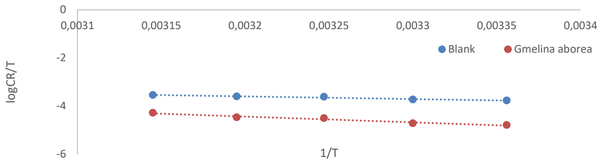
Figure 1. Arrhenius plot
